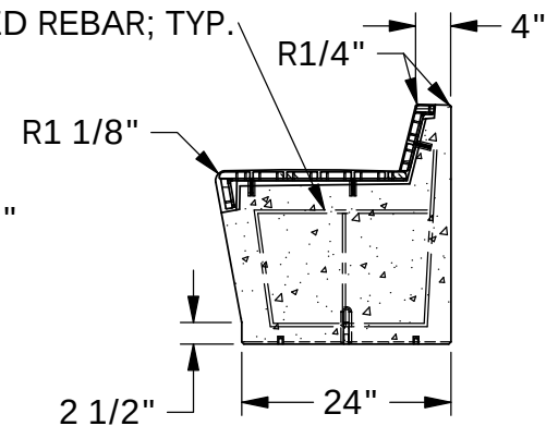
⑤ SECTION
