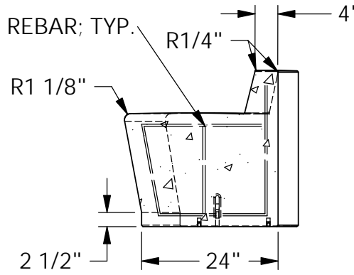
⑤ SECTION
