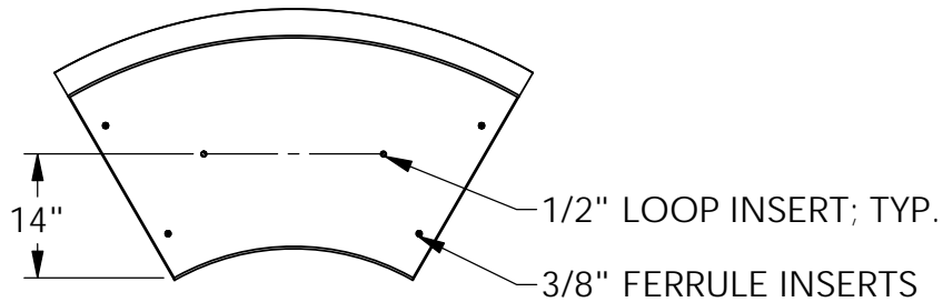
③ BOTTOM VIEW
