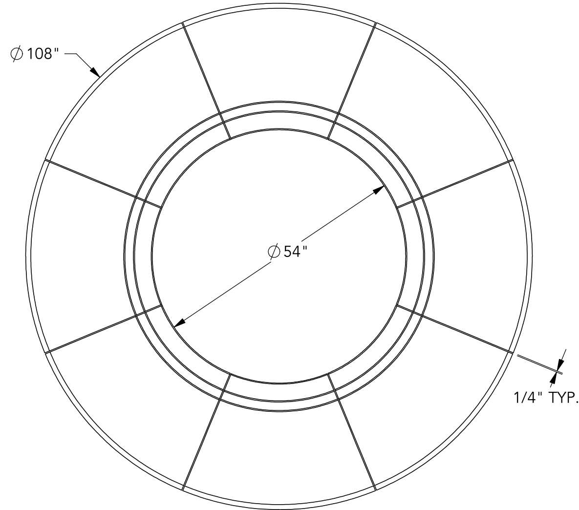
1 TOP VIEW (QTY. 8)
