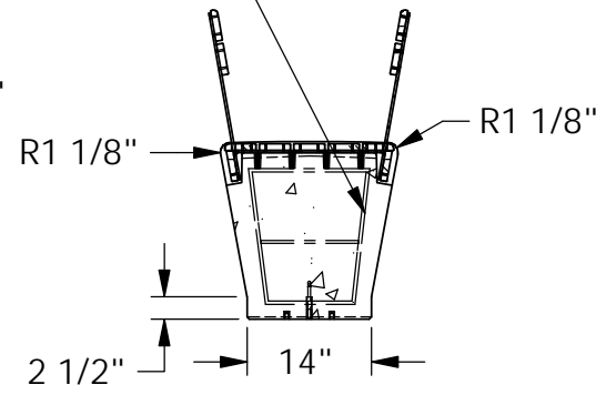
⑤ SECTION
