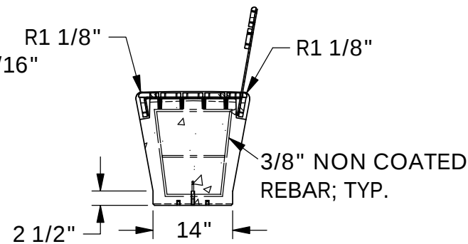
⑤ SECTION
