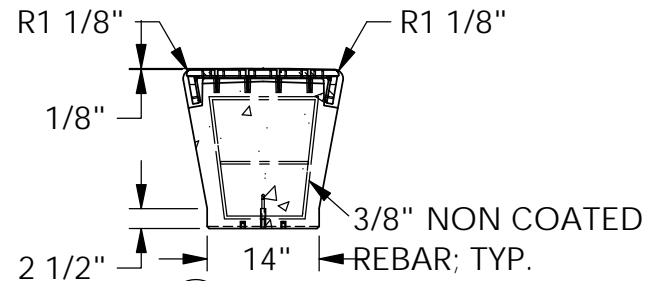
⑤ SECTION
