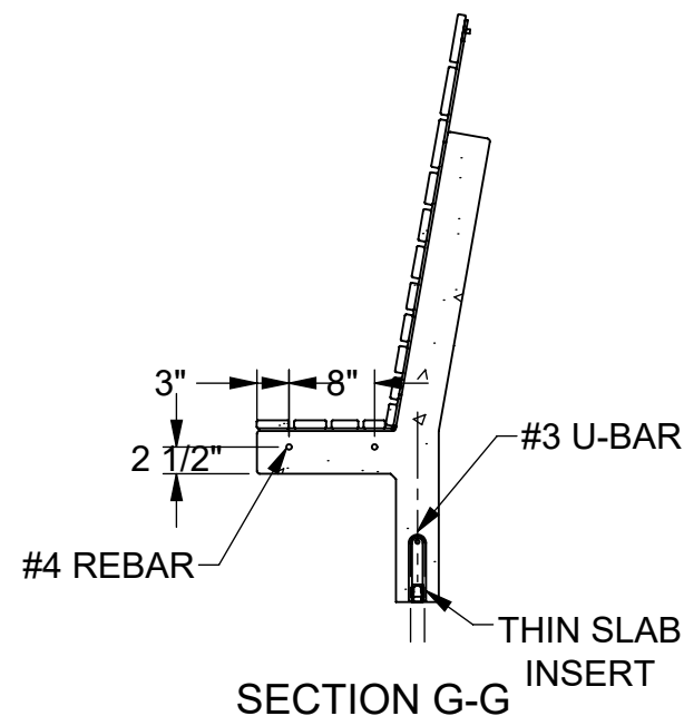
④ SECTION
