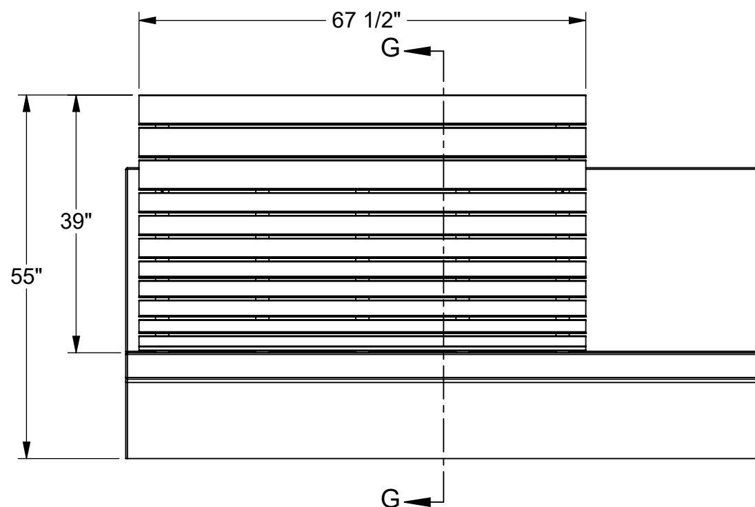
② FRONT VIEW
