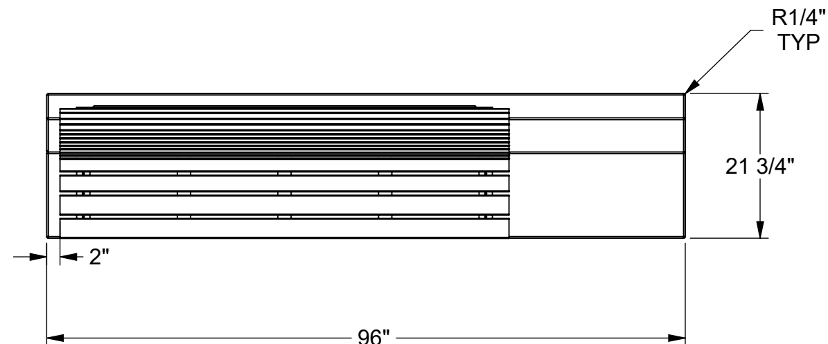
① TOP VIEW
