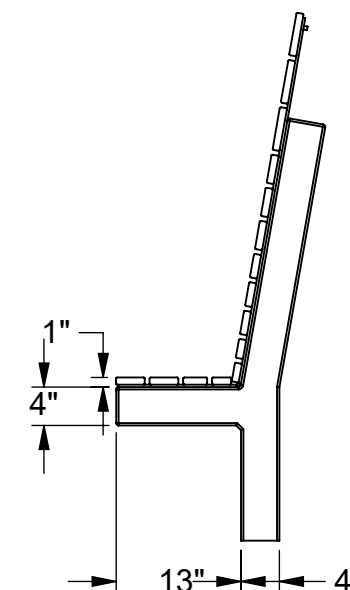
⑥ RIGHT SIDE
