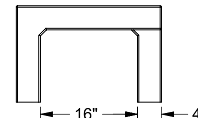
⑥ RIGHT SIDE
