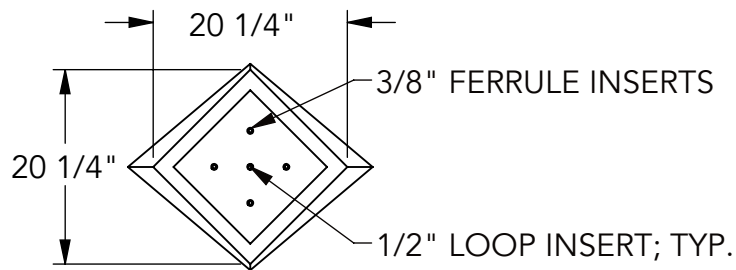
③ BOTTOM VIEW
