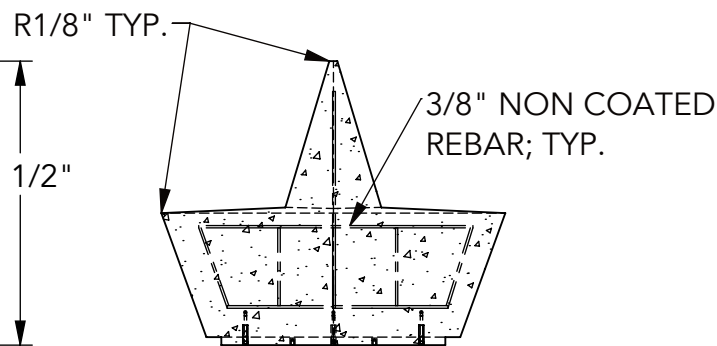
⑤ SECTION
