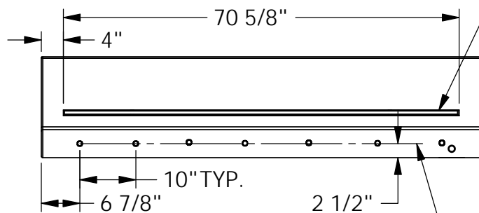
③ BOTTOM VIEW
