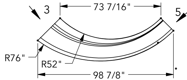
① TOP VIEW
