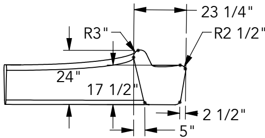
③ SIDE VIEW
