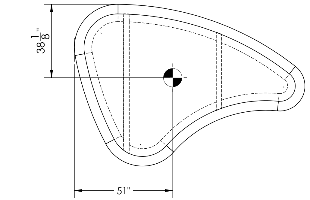
① TOP VIEW
