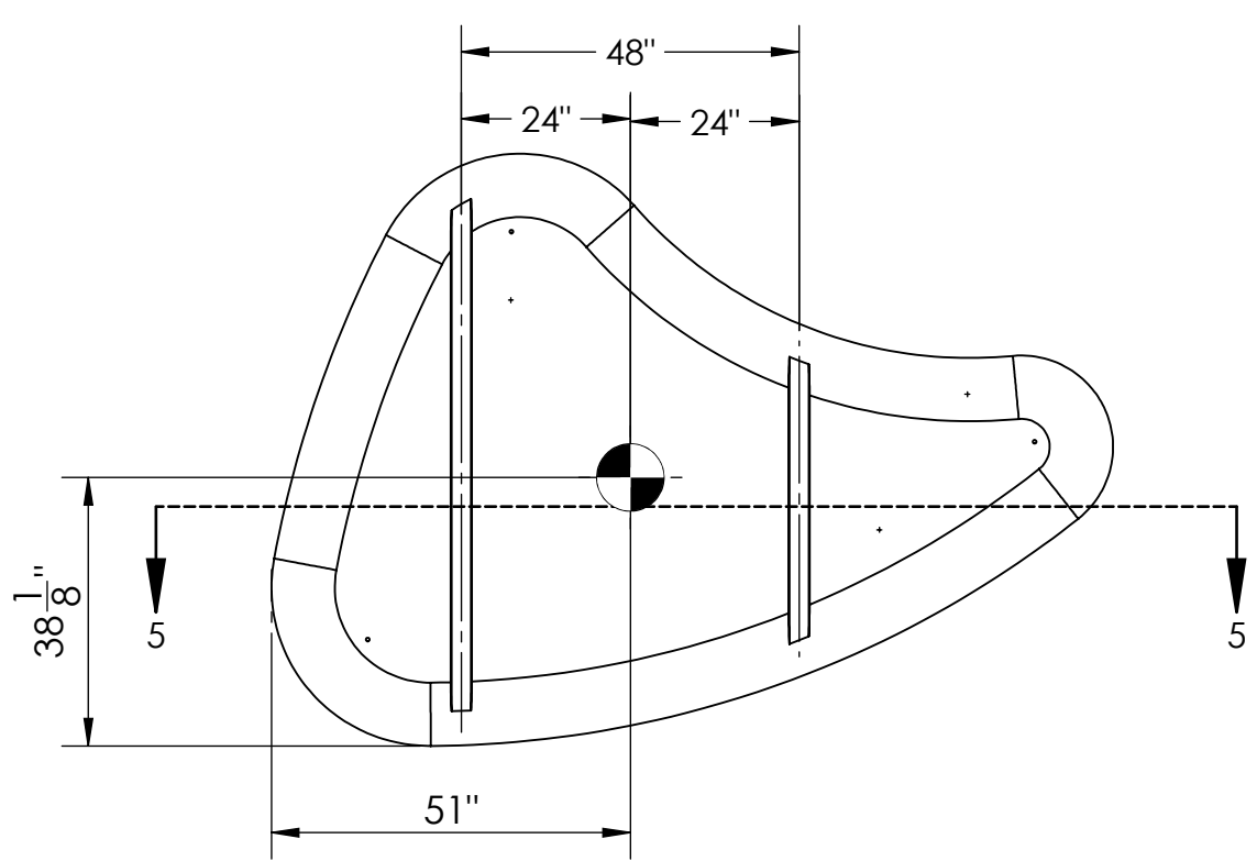
③ BOTTOM VIEW
