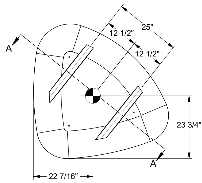
③ BOTTOM VIEW
