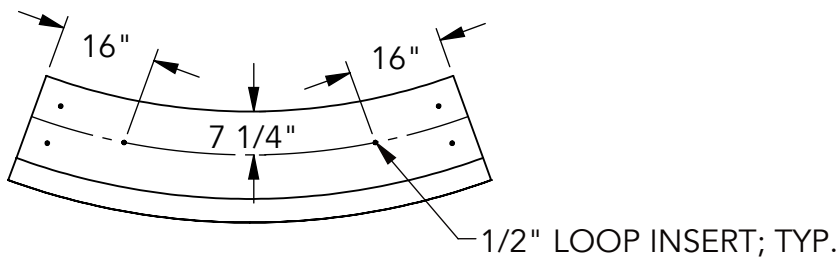
③ BOTTOM VIEW
