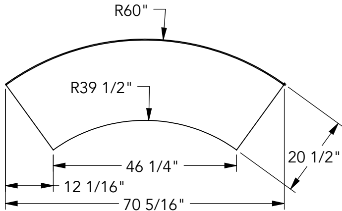
① TOP VIEW
