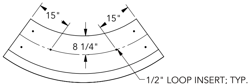
③ BOTTOM VIEW
