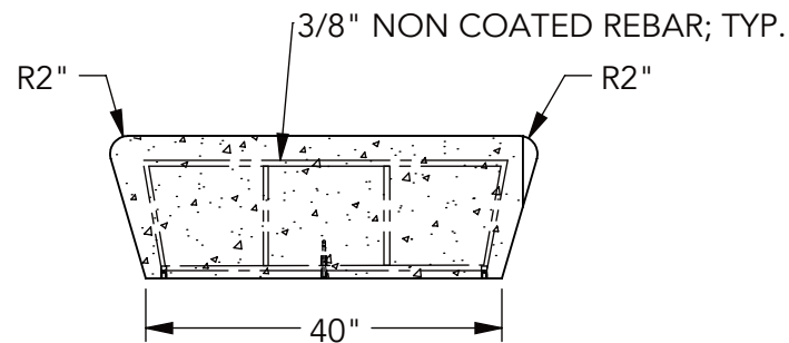
⑤ SECTION
