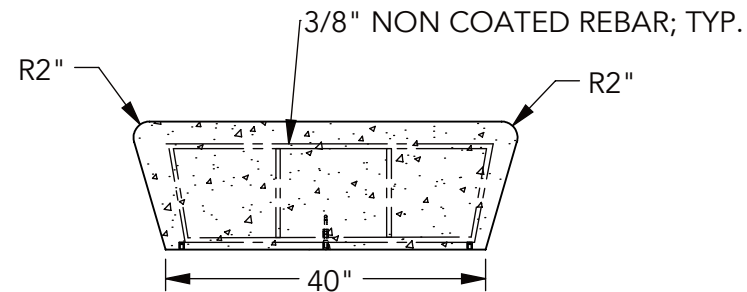
⑤ SECTION
