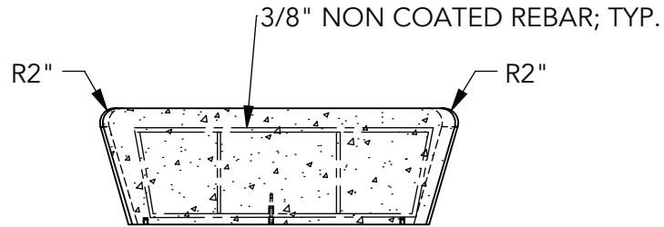
⑤ SECTION
