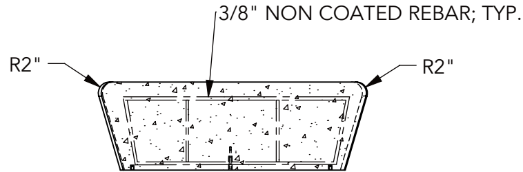
⑤ SECTION
