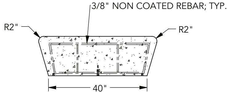
⑤ SECTION
