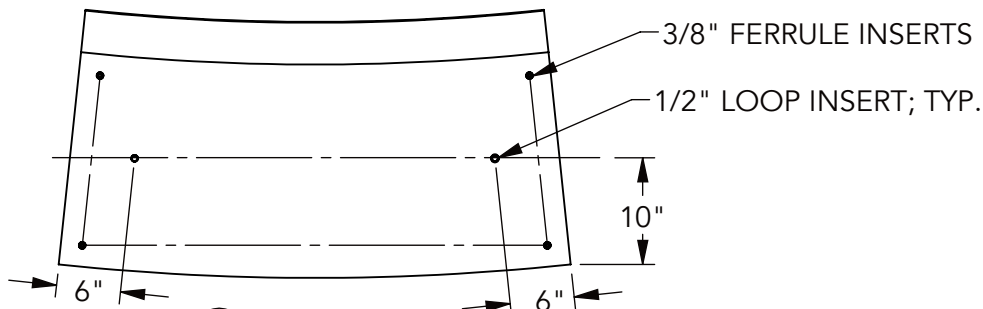
③ BOTTOM VIEW
