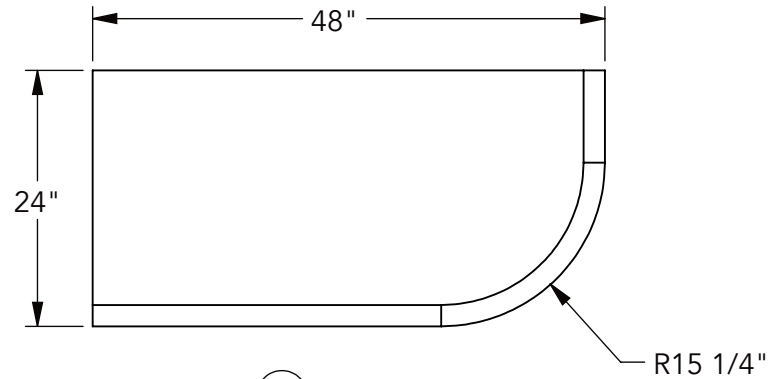
① TOP VIEW
