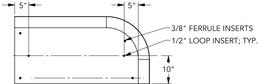
③ BOTTOM VIEW
