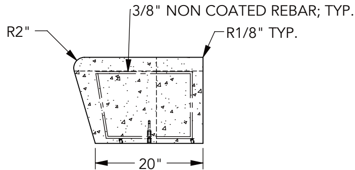
⑤ SECTION
