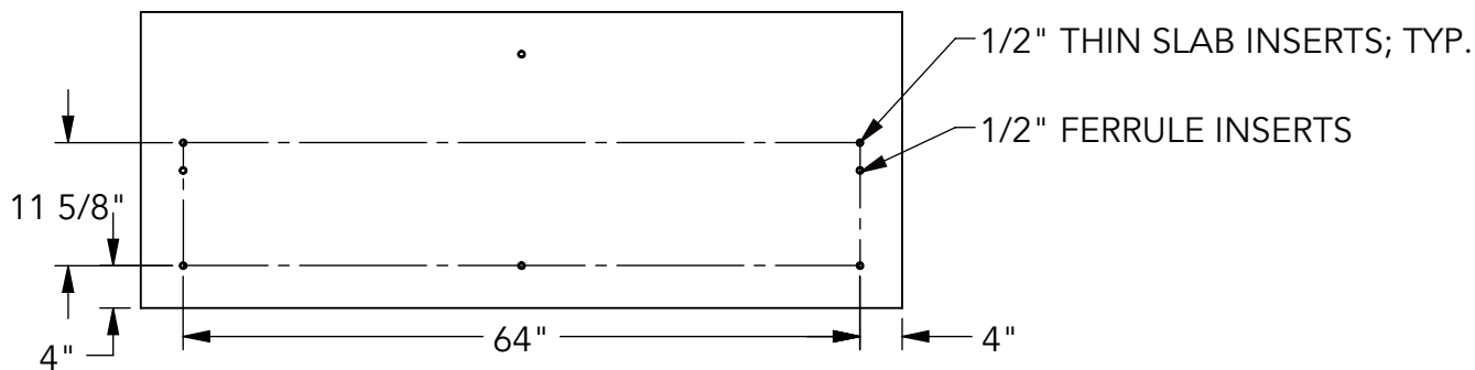
③ BOTTOM VIEW
