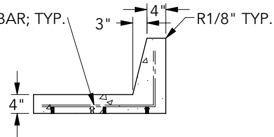
⑤ SECTION
