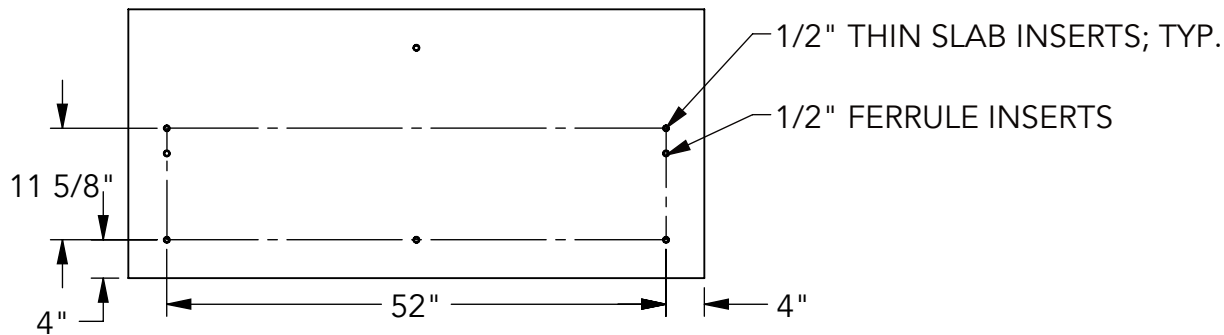
③ BOTTOM VIEW
