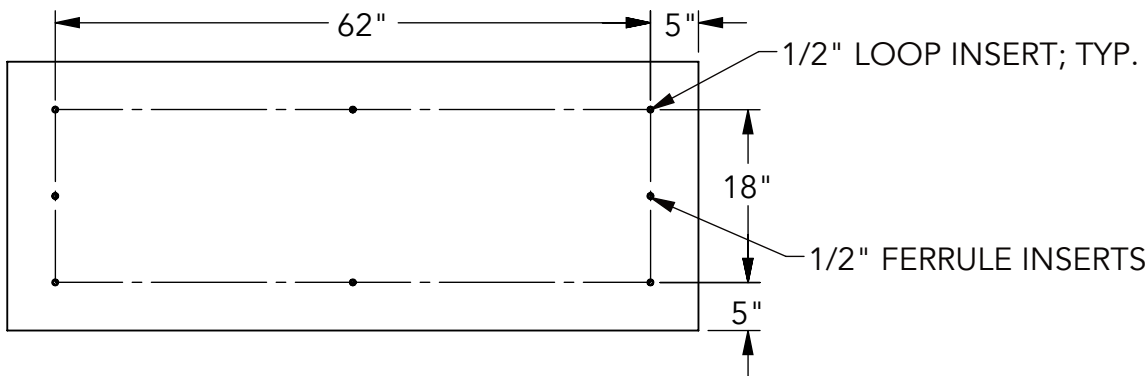
3 BOTTOM VIEW
