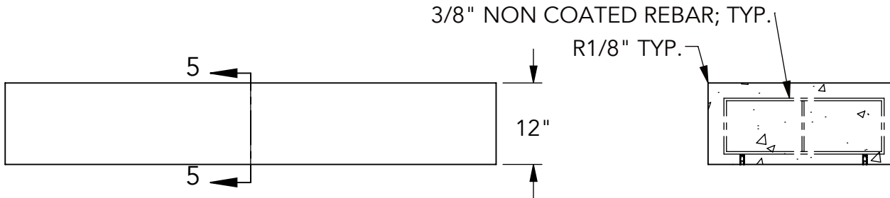
5 SECTION
