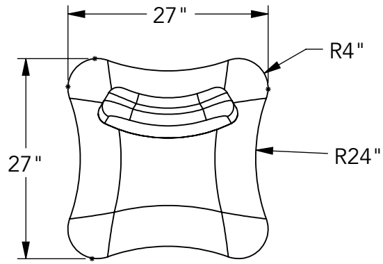
① TOP VIEW
