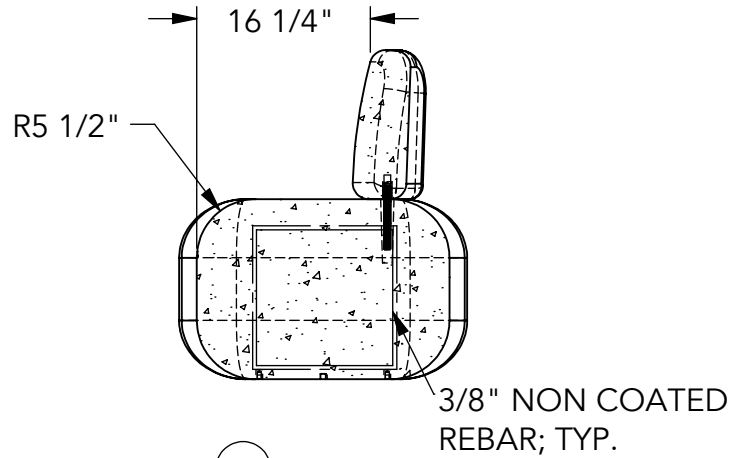
⑤ SECTION
