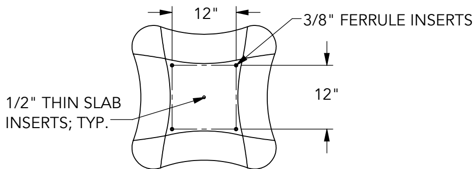
③ BOTTOM VIEW
