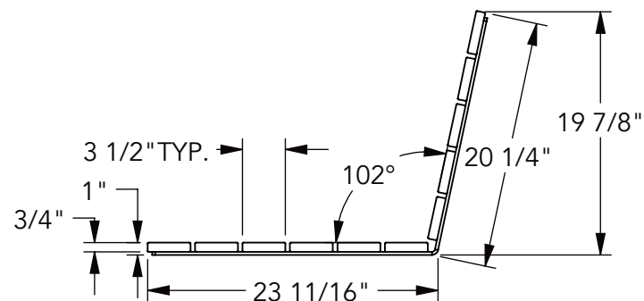
4 SIDE VIEW
