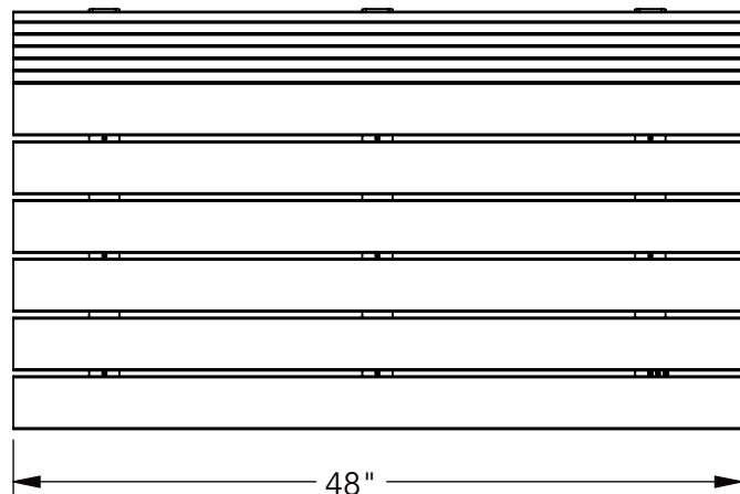
1 TOP VIEW
