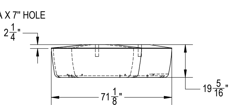
4 SIDE VIEW
