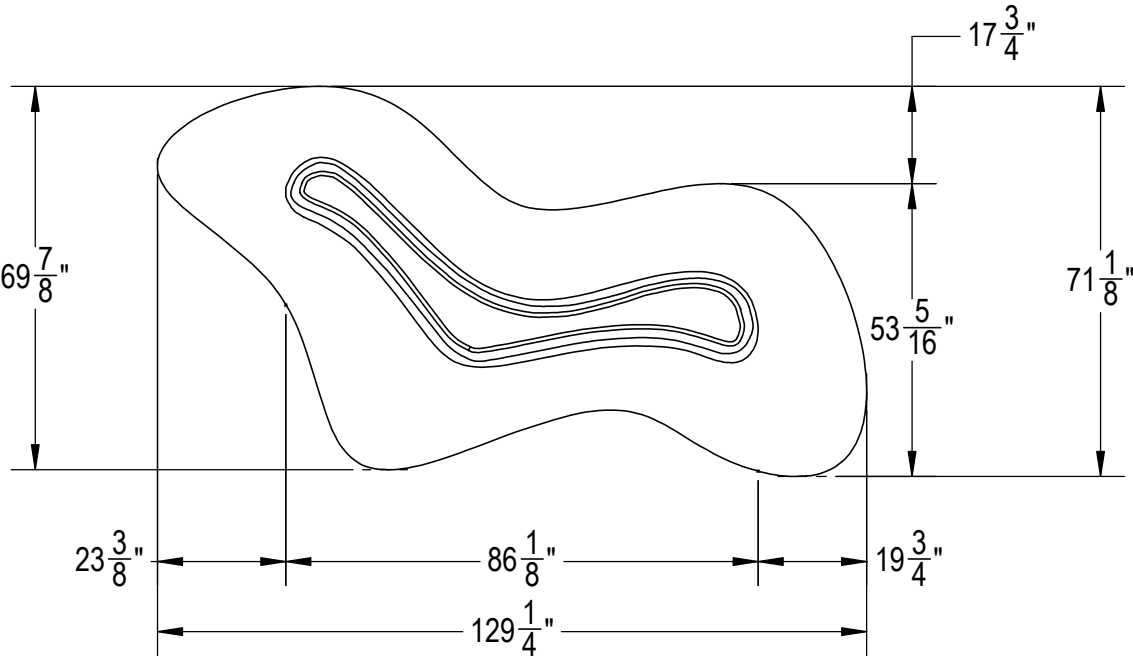
① TOP VIEW
