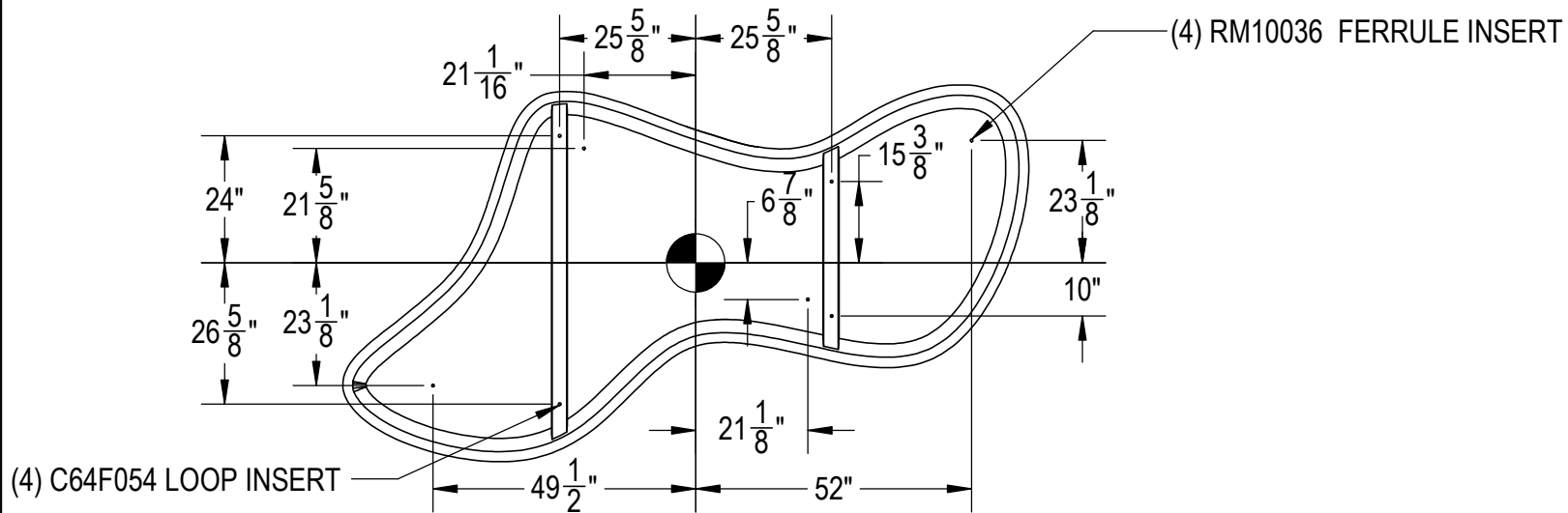
3 BOTTOM VIEW
