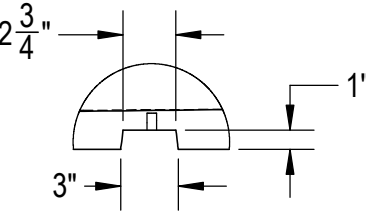
⑤ DETAIL A
