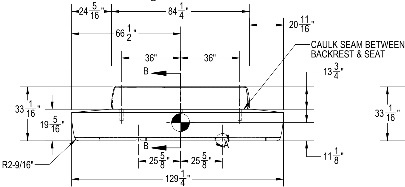
② FRONT VIEW
