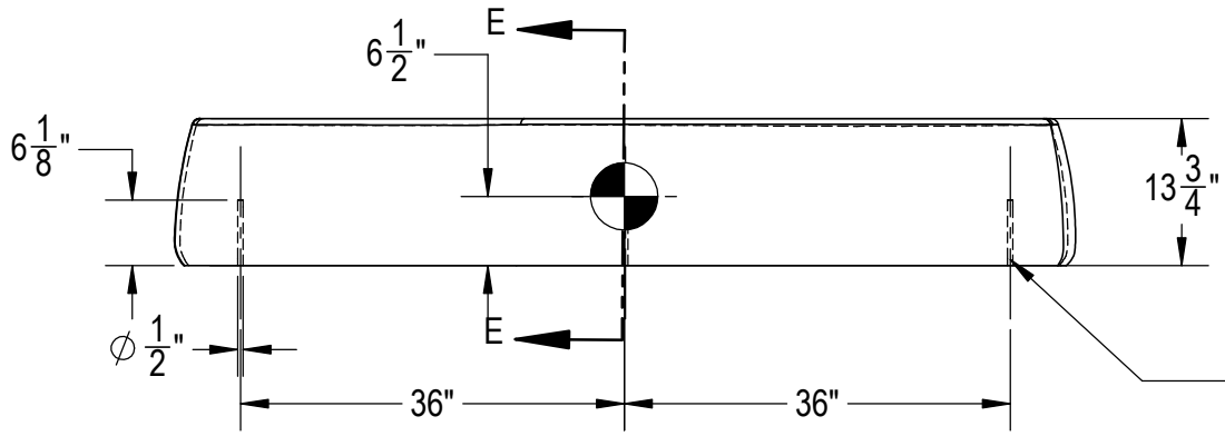
2 FRONT VIEW
