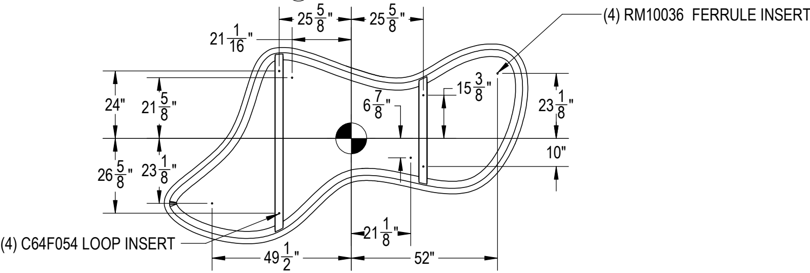
③ BOTTOM VIEW
