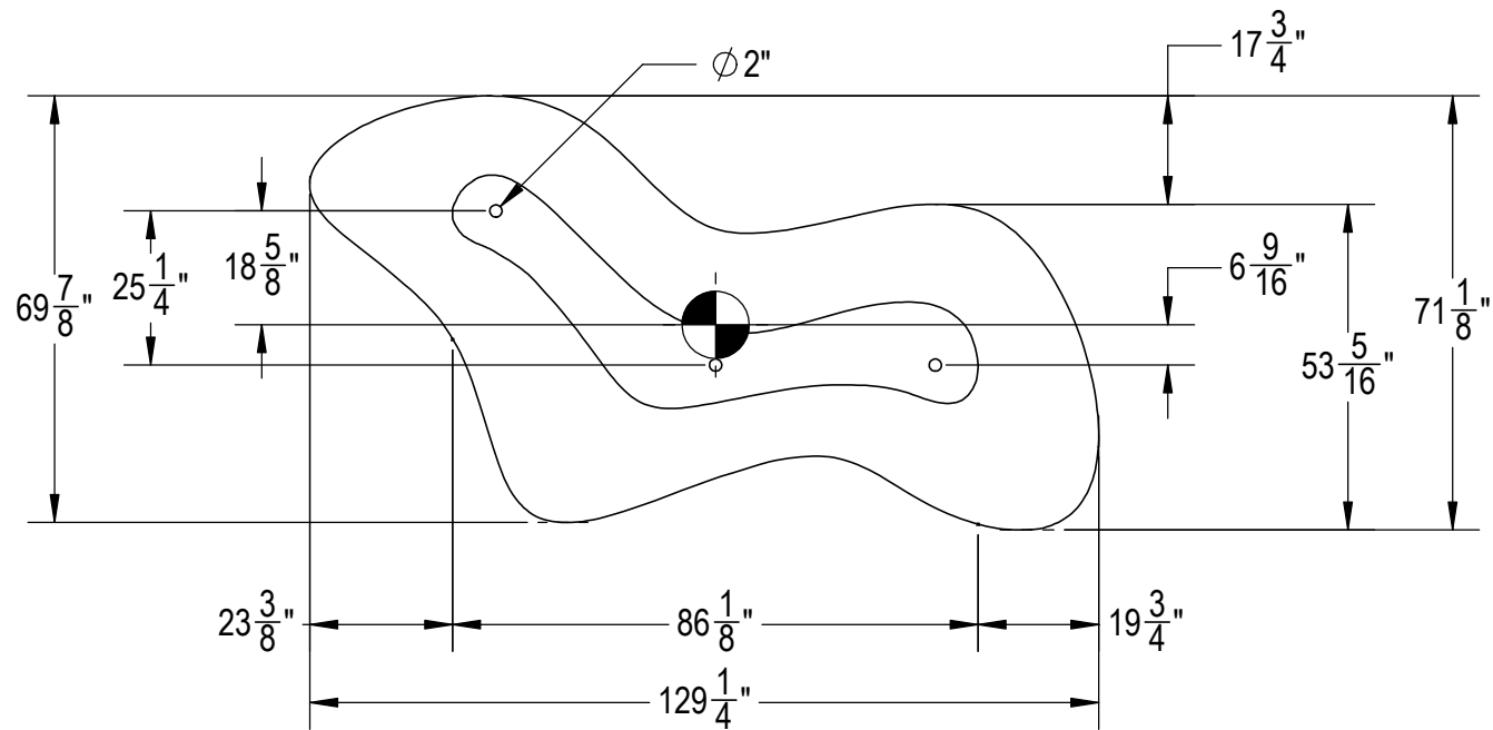
1 TOP VIEW
