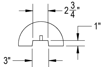
5 DETAIL D
