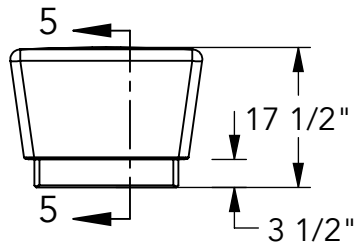
2 FRONT VIEW
