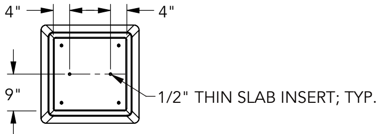
3 BOTTOM VIEW
