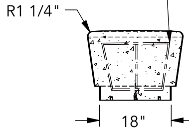
5 SECTION
