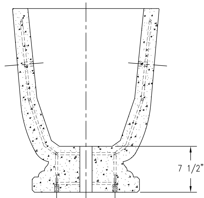
4 CROSS SECTION
