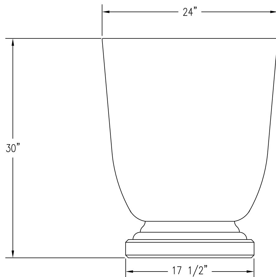
2 ELEVATION VIEW
