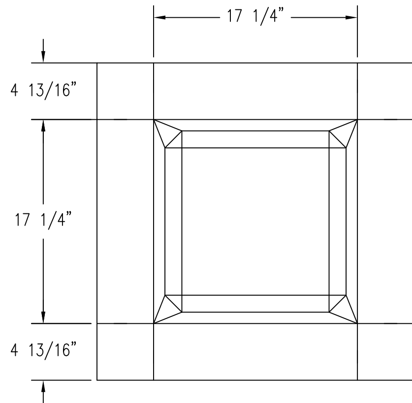
1 TOP VIEW
