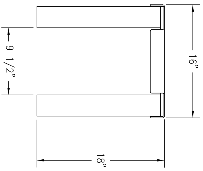
2 WS-215, ELEVATION Scale: 1/8" = 1"
