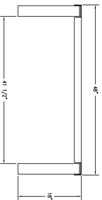
2 SIDE ELEVATION OF WS-214 BENCH Scale: 1/8" = 1"
