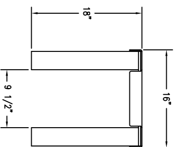
3 SIDE ELEVATION OF WS-214 BENCH Scale: 1/8" = 1"
