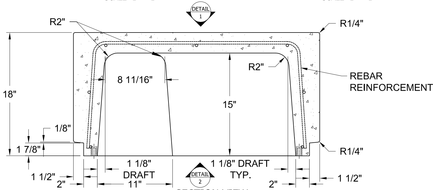
6 SECTION VIEW SCALE: 1 1/2" = 1'
