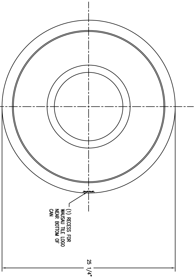
3 TOP VIEW
