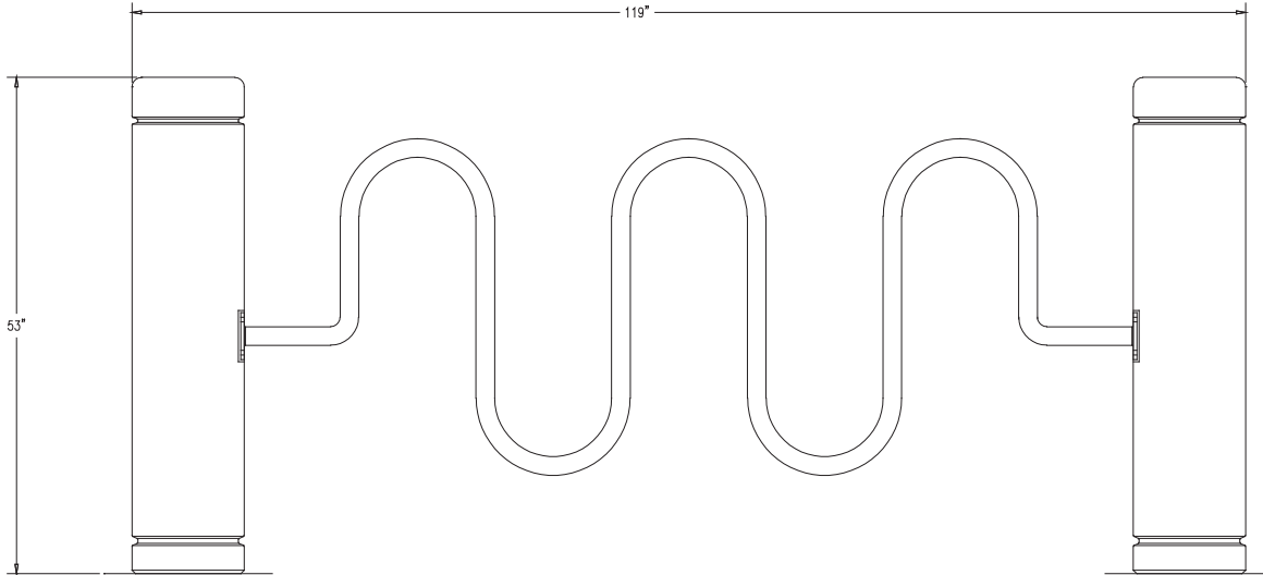
ELEVATION VIEW
