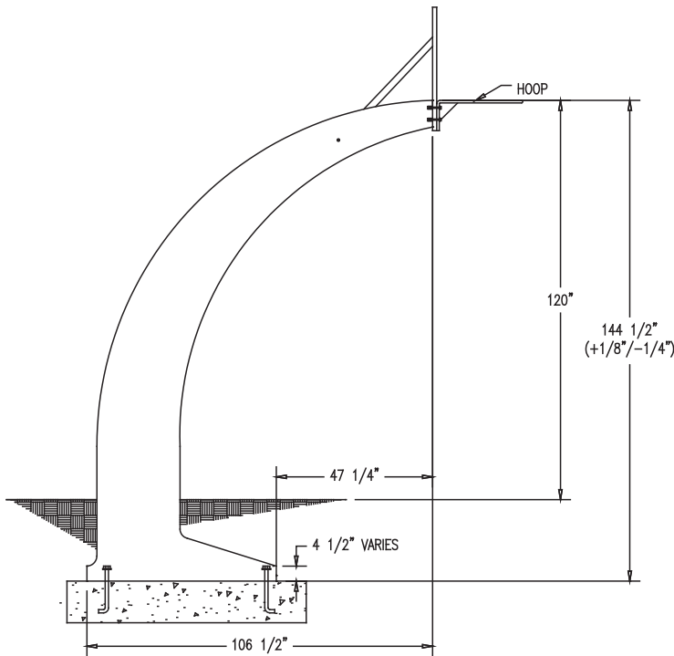
ELEVATION VIEW
