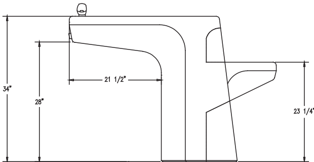
ELEVATION VIEW
