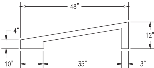
ELEVATION VIEW
