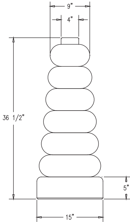
ELEVATION VIEW
