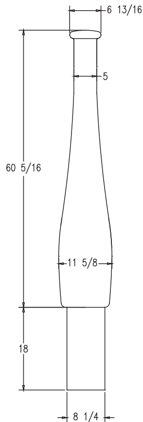
ELEVATION VIEW
