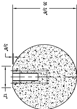
4 CROSS SECTION
