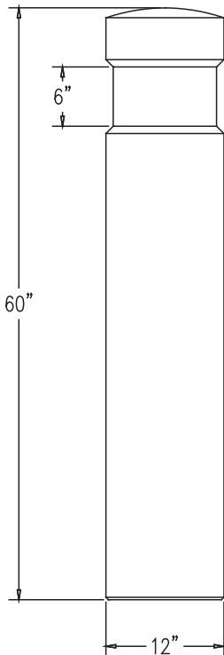
ELEVATION VIEW
