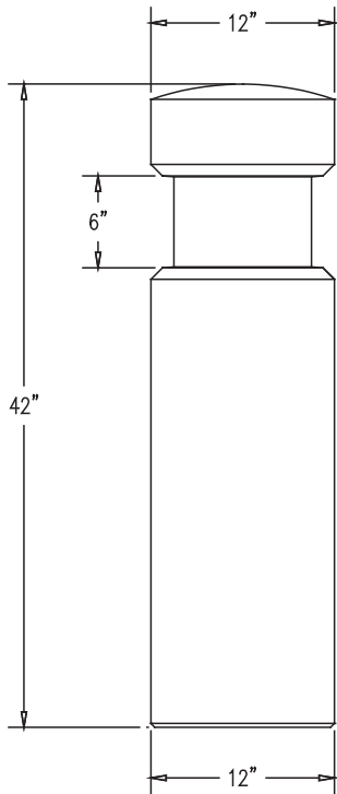
ELEVATION VIEW
