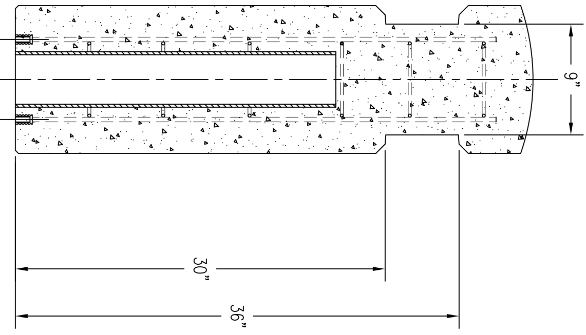
4 CROSS SECTION
