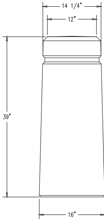
ELEVATION VIEW
