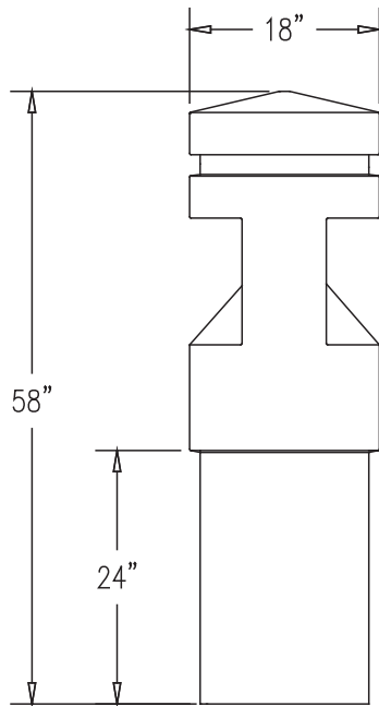
ELEVATION VIEW
